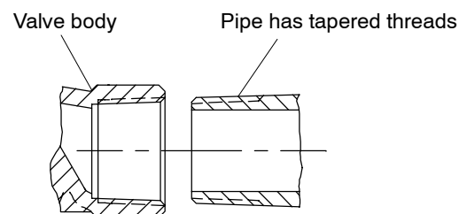
Fig. 25. 3/4" BSPT internal (Rc 3/4) or NPT internal
