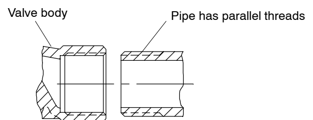
Fig. 24. 3/4" BSPP internal (Rp 3/4)
