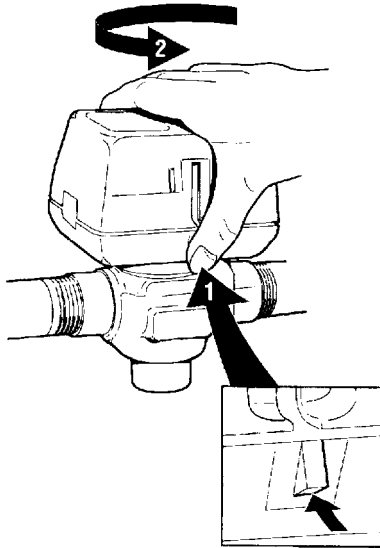
Fig. 11. Latch mechanism
